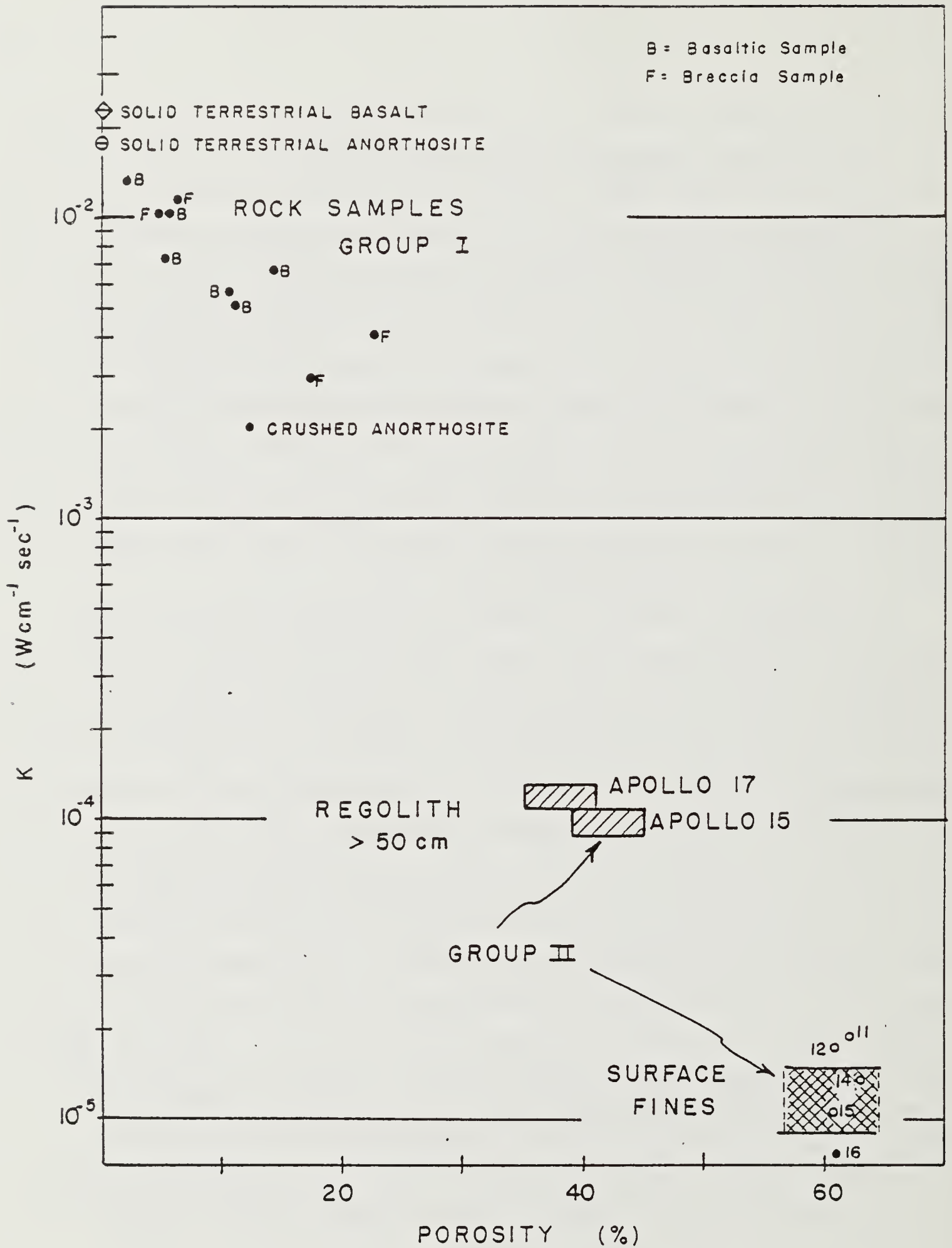
Published conductivity values of lunar materials vs. porosity. For laboratory measurements, values at 300°K are shown as points in the plot. The doubly hatched box is the range of in situ values determined from nighttime cooldown data (Keihm and Langseth, 1973) and the singly hatched boxes are the results reported in this paper. Rock data are summarized in Horai and Winkler (1976) and soil data in Cremers and Hsia (1973)
